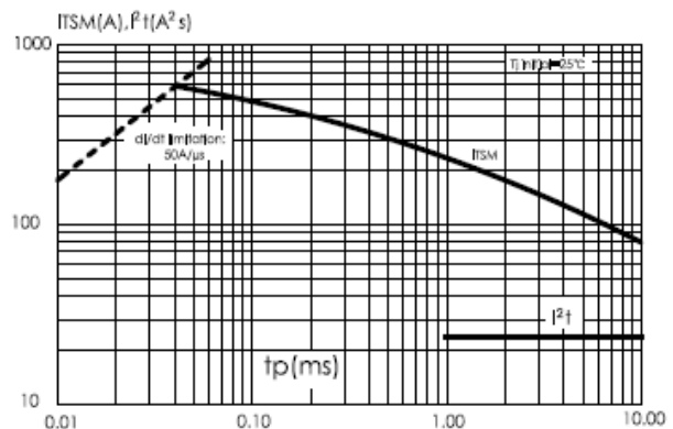
Fig. 4: Non-repetitive surge peak on-state current for a sinusoidal pulse with width t_p < 10 ms, and corresponding value of I^2t .
